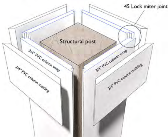
PVC COLUMN WRAP 3D VIEW
