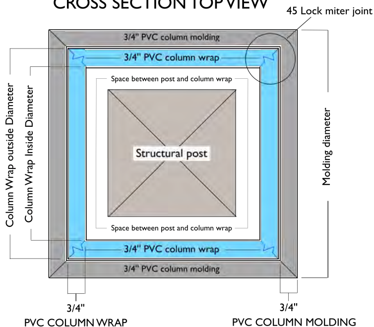
CROSS SECTION TOP VIEW
